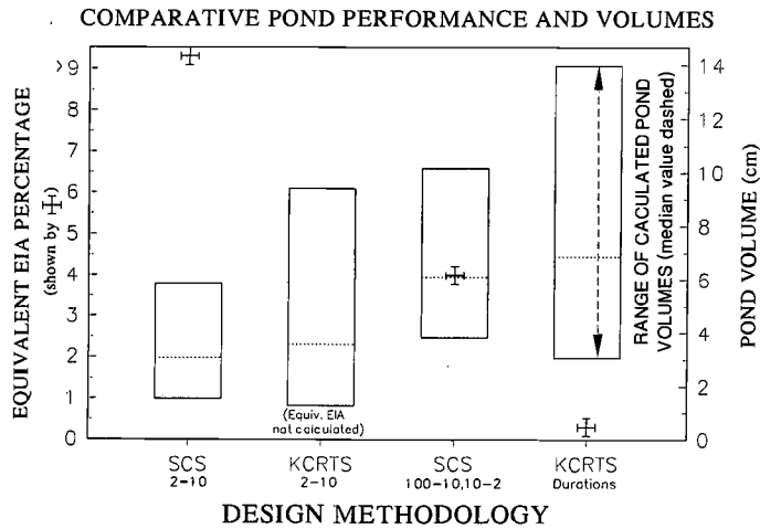
Figure 6. Comparative pond performance using different design methodologies – SCS and KCRTS hydrologic models, each under peak (labeled “2-10”) and duration (labeled “100-10,10-2” or “Durations”) standards. Evaluations are based on HSPF simulations of different developments within the fully built-out Soosette Creek watershed (29 percent impervious; see Figure 1). Overall performance (crosses) is represented by the equivalent flow increases allowed by a watershed having the indicated impervious-area percentage (as EIA) without detention; only KCRTS with a duration standard achieves “full” mitigation. The range of pond sizes (boxes) is expressed in cm-ha of volume per developed ha, with the range imposed by variability of soils and pre-development vegetation and the median value for all simulations shown by the dotted line.
