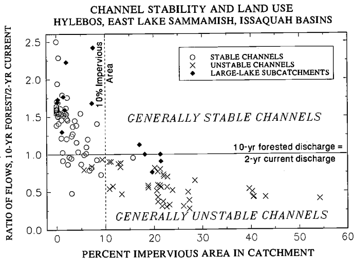
Figure 4. Observed stable (“O”) and unstable (“X”) channels, plotted by percent effective impervious area (EIA) in the upstream watershed (horizontal scale) and ratio of modeled 10-year forested and two-year current (i.e. urbanized) discharges (vertical scale). Apparent thresholds relating channel stability with either 10 percent EIA or Q_{2-cur} = Q_{10-for} are consistently met except for the few catchments containing large lakes.
