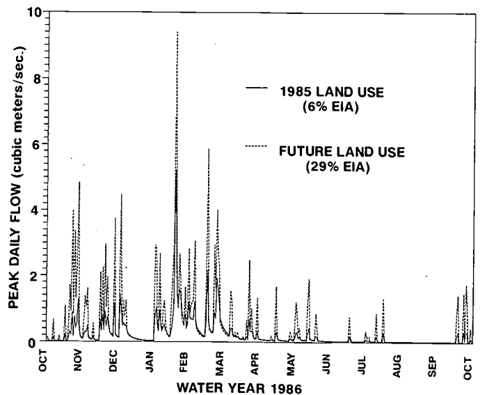
Figure 2. One year of simulated streamflow from a 14.2-km 2 watershed (Soosette Creek), under identical rainfall but differing land uses, using the continuous numerical model HSPF (USEPA, 1984). Parameters characterize the present-day (1985) land cover [6 percent effective impervious area (EIA), the impervious surfaces with direct hydraulic connection to the stream system] and projected future land cover (29 percent EIA).
