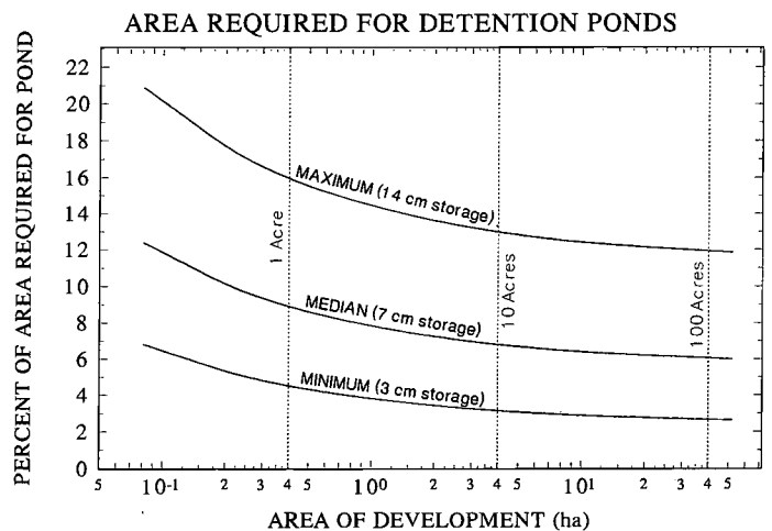
Figure 7. Relative gross area required for detention ponds, depending on the development area and the desired volume of stored runoff (expressed as cm-ha per ha of developed land). Pond layout and design is in accord with local regulations and assumes a 1.3-m (4-ft) maximum water depth and 3:1 sideslopes on all confining berms. Range of pond volumes correspond to the likely values determined with a “KCRTS duration” standard (Figure 6).
